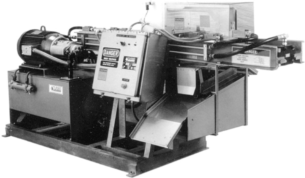
BP240 with Standard Block Bagger
